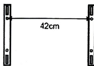
Varianten 650mm
