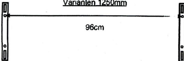
Varianten 1250mm
