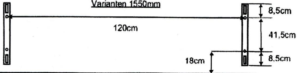
Varianten 1550mm
